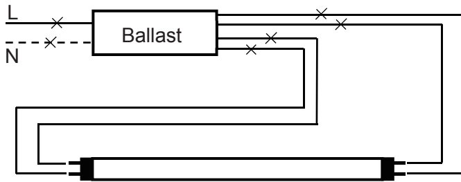
Step 1. Cut all wires connected to the existing ballast, remove the ballast.
