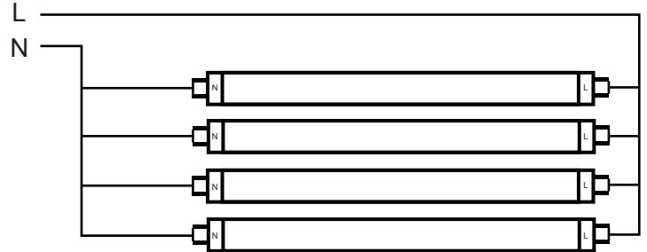
Step 2. Connect the lamps according to the above wiring diagram
