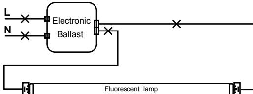
Instant Start (Shunted Socket) Configuration
